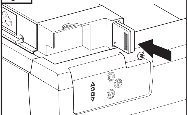
Fig. 35 Modular Antenna Installation or Replacement
