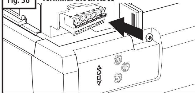
Terminal block XB03
